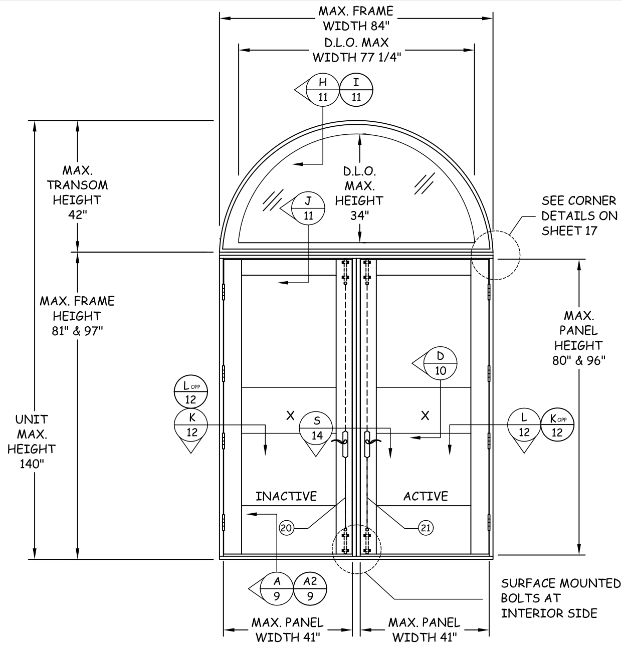
O/XX W/ TRANSOM CONFIGURATION SEE DESIGN PRESSURE TABLE EXTERIOR ELEVATION OUTSWING DOUBLE OPAQUE DOORS W/ TRANSOM
