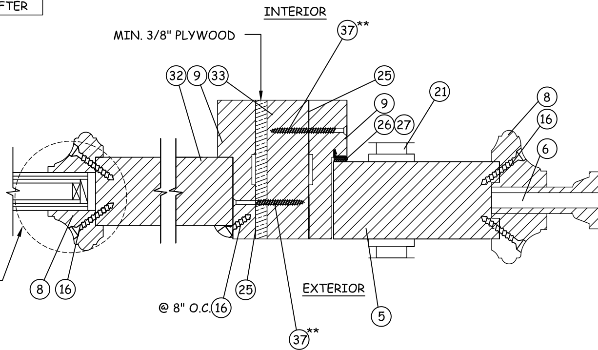
R13 HORIZONTAL SECTION VERTICAL MULLION SIDELITE/MULLION/HINGE JAMB
