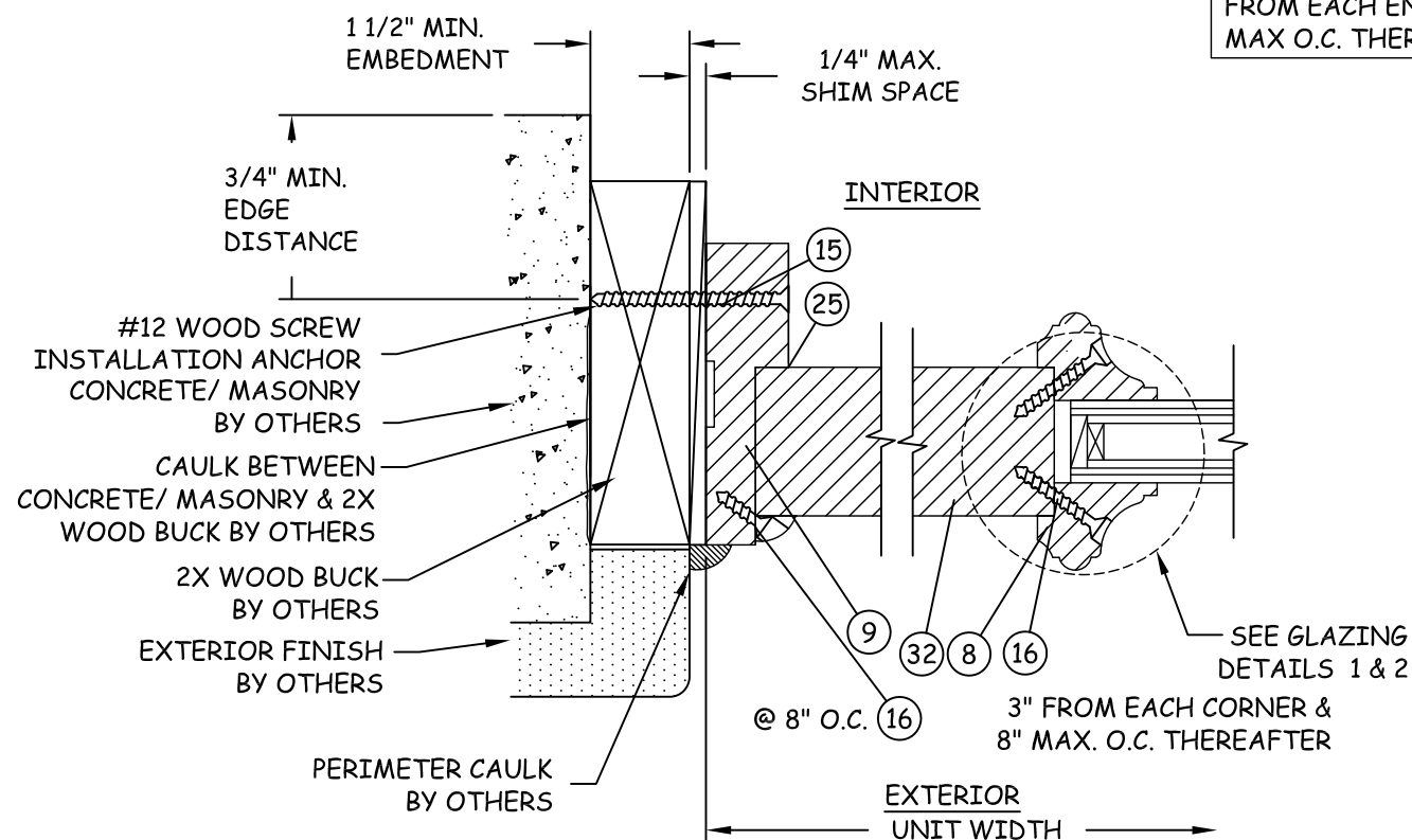
O13 HORIZONTAL SECTION SIDELITE JAMB AT 2 WOOD BUCK
