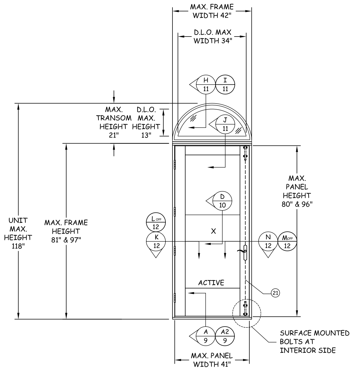
O/X W/ TRANSOM CONFIGURATION SEE DESIGN PRESSURE TABLE EXTERIOR ELEVATION OUTSWING SINGLE OPAQUE DOOR W/ TRANSOM
