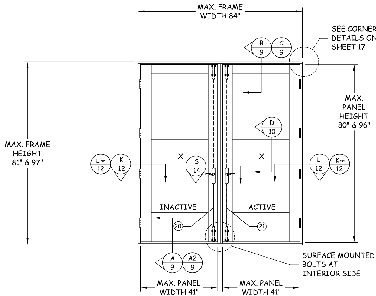
XX CONFIGURATION SEE DESIGN PRESSURE TABLE EXTERIOR ELEVATION OUTSWING DOUBLE OPAQUE DOOR
