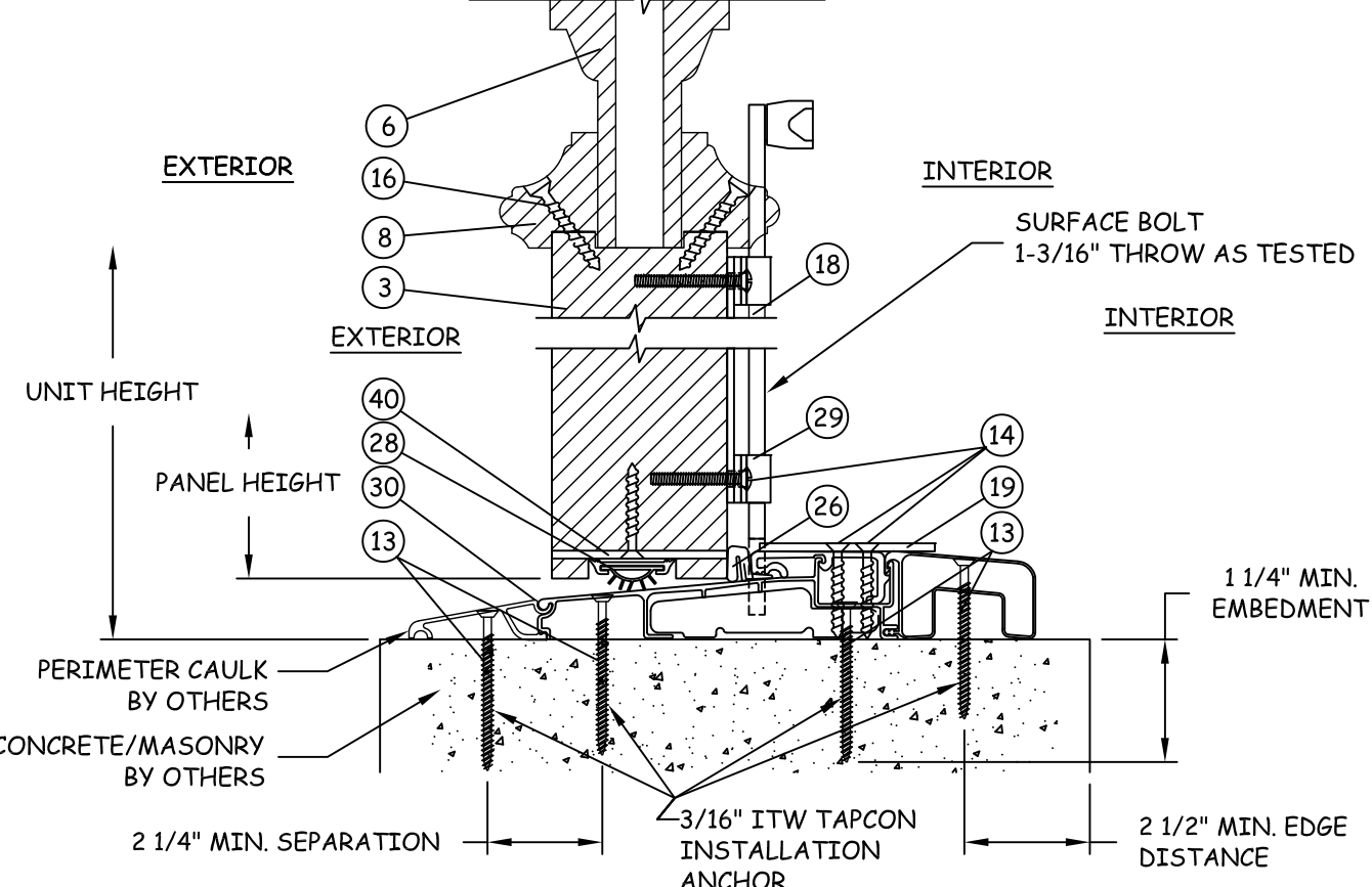
A 9 VERTICAL SECTION DOOR SILL - CONCRETE/MASONRY
