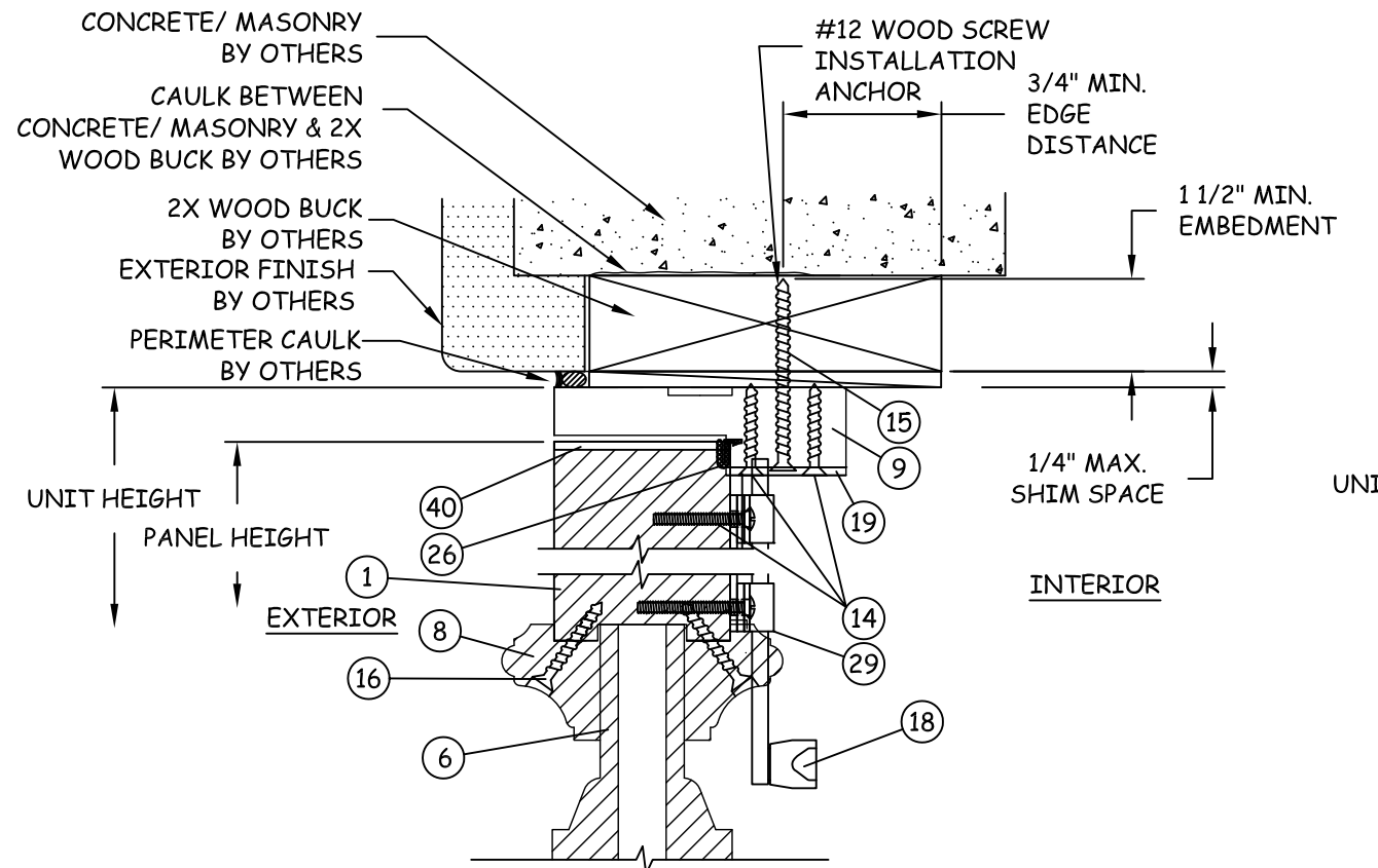
B 9 VERTICAL SECTION DOOR HEAD AT 2X WOOD BUCK
