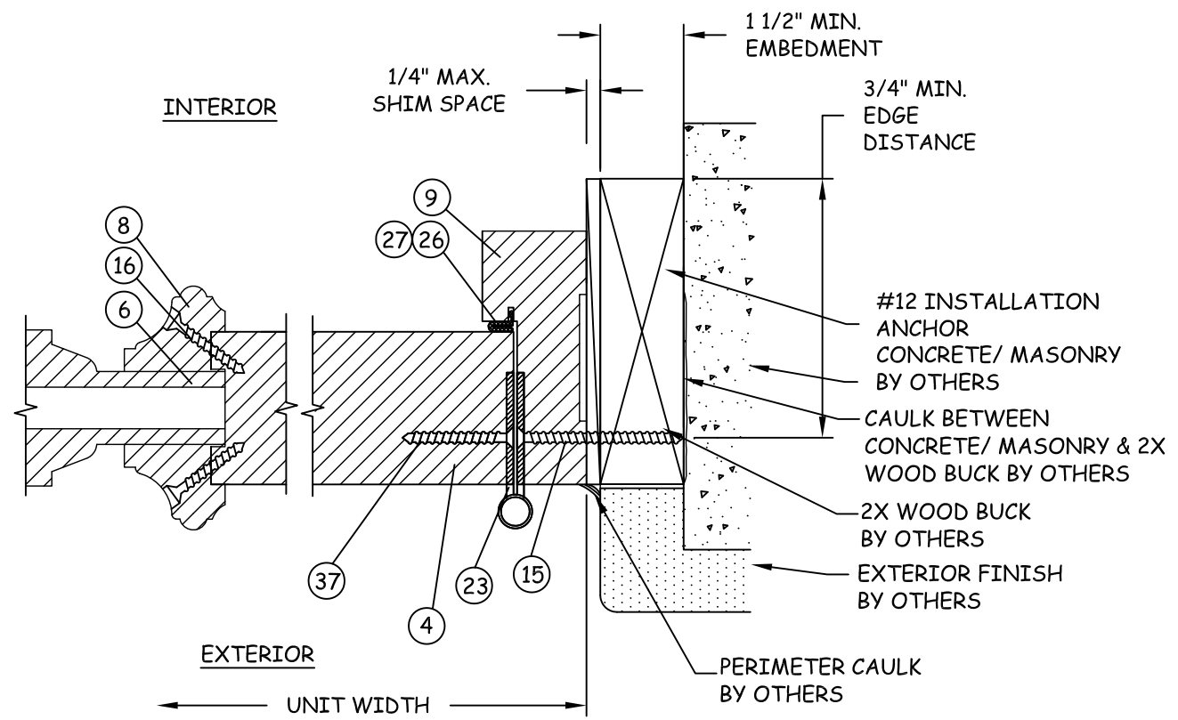
L 12 HORIZONTAL SECTION DOOR HINGE JAMB AT 2X WOOD BUCK
