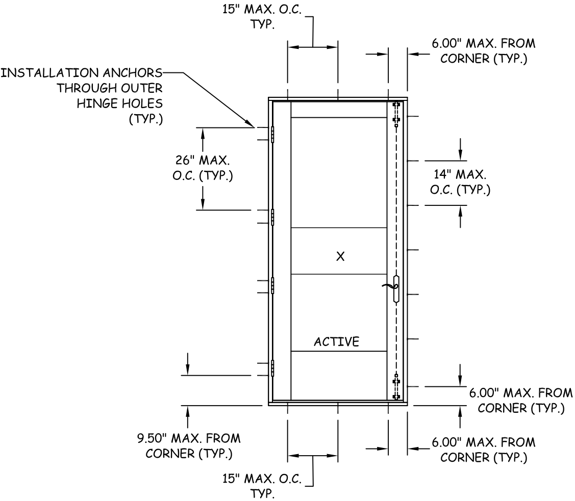
ANCHOR LAYOUT
