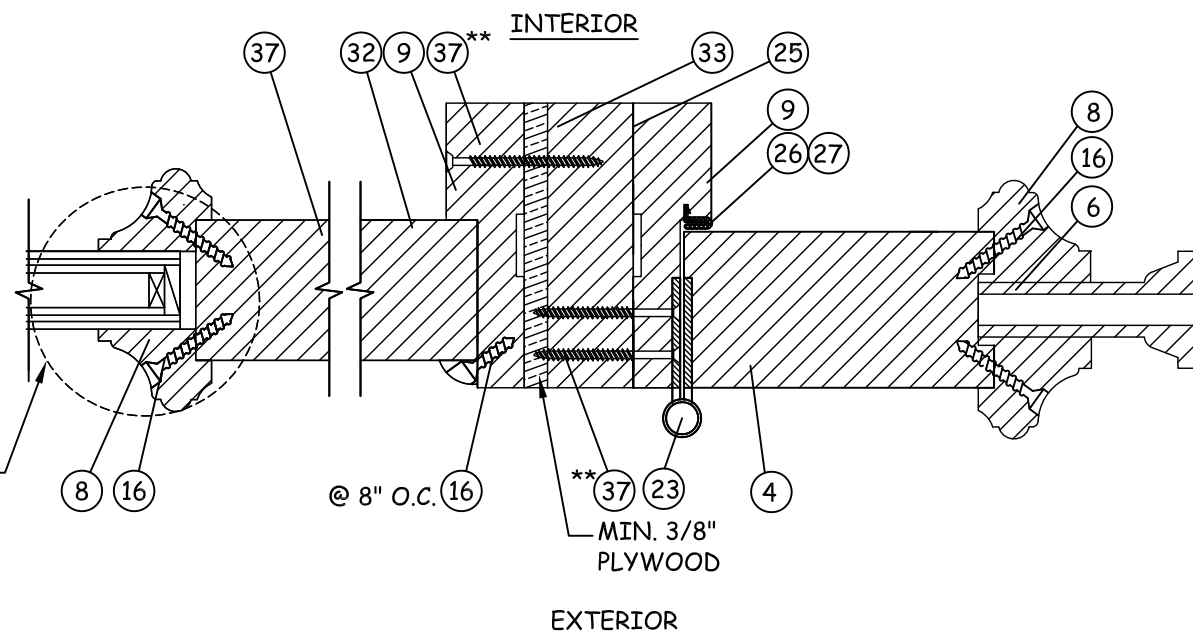
R13 HORIZONTAL SECTION VERTICAL MULLION SIDELITE/MULLION/HINGE JAMB
