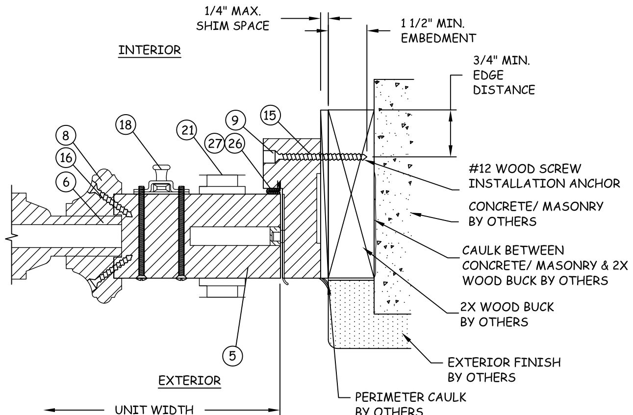
N 12 HORIZONTAL SECTION LOCK JAMB AT 2X WOOD BUCK
