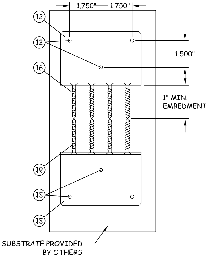
SIDE VIEW HORIZONTAL MULLION DETAIL
