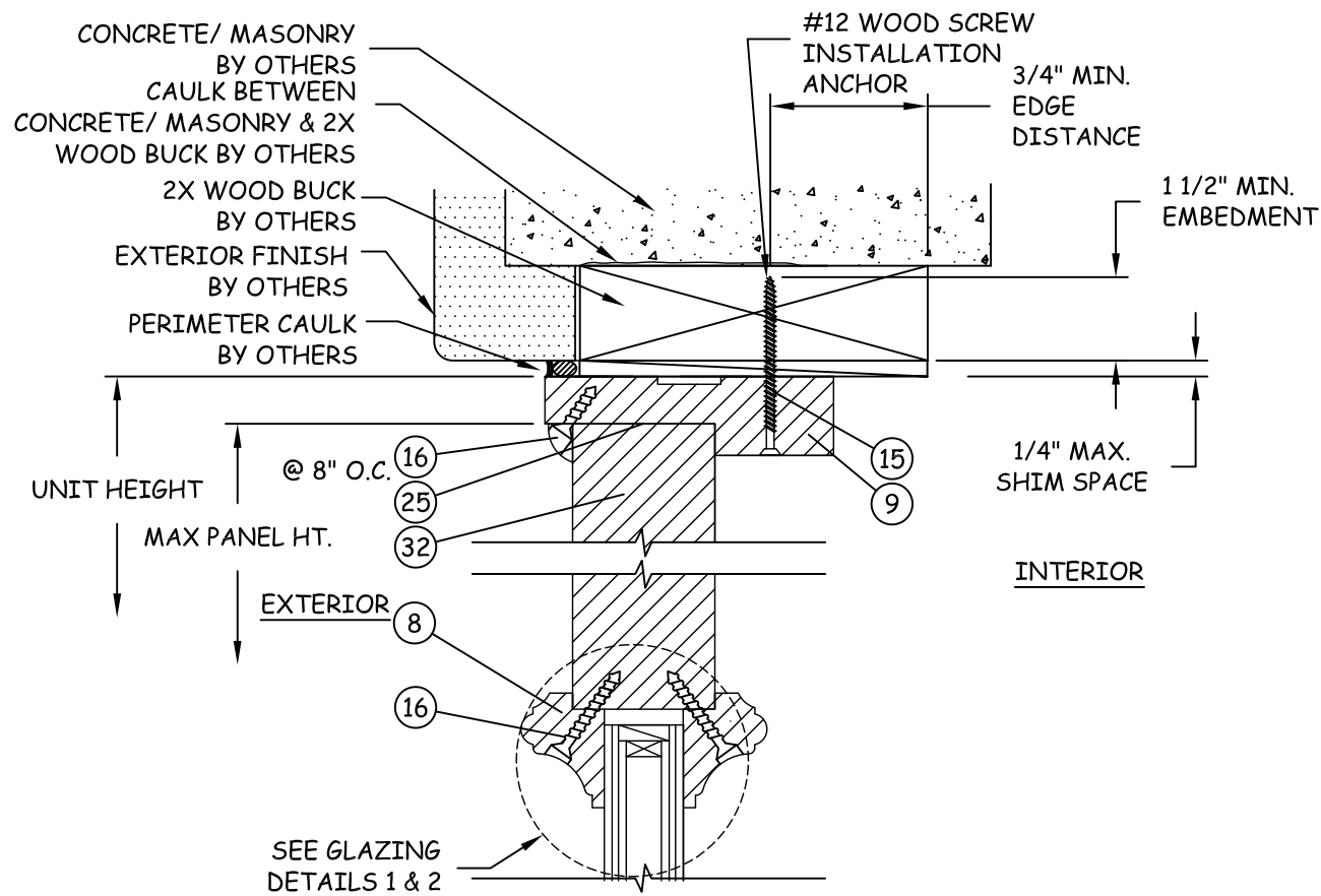
F 10 VERTICAL SECTION SIDELITE HEAD AT 2X WOOD BUCK
