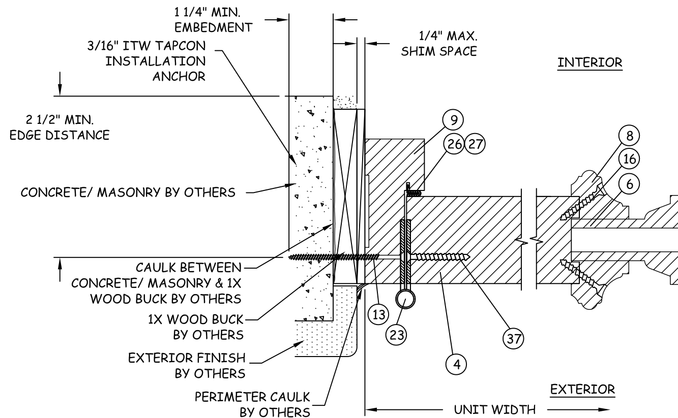
K 12 HORIZONTAL SECTION DOOR HINGE JAMB AT CONCRETE/MASONRY
