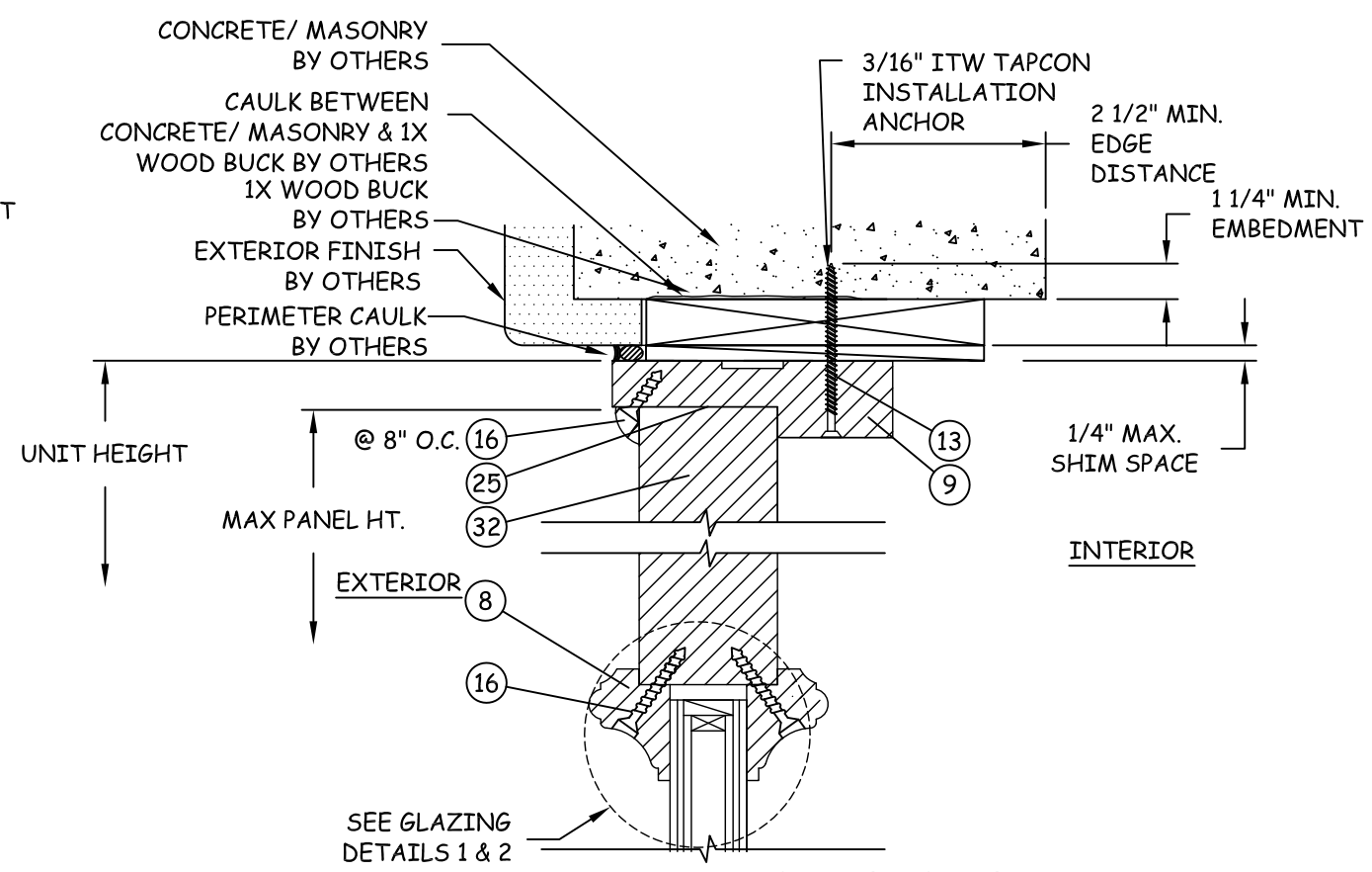
G 10 VERTICAL SECTION SIDELITE HEAD AT CONCRETE/MASONRY
