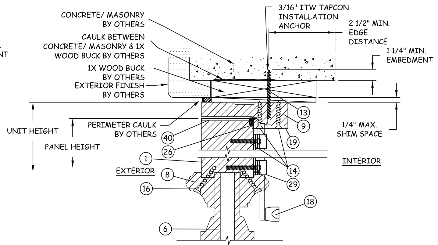
C 9 VERTICAL SECTION DOOR HEAD AT CONCRETE/MASONRY
