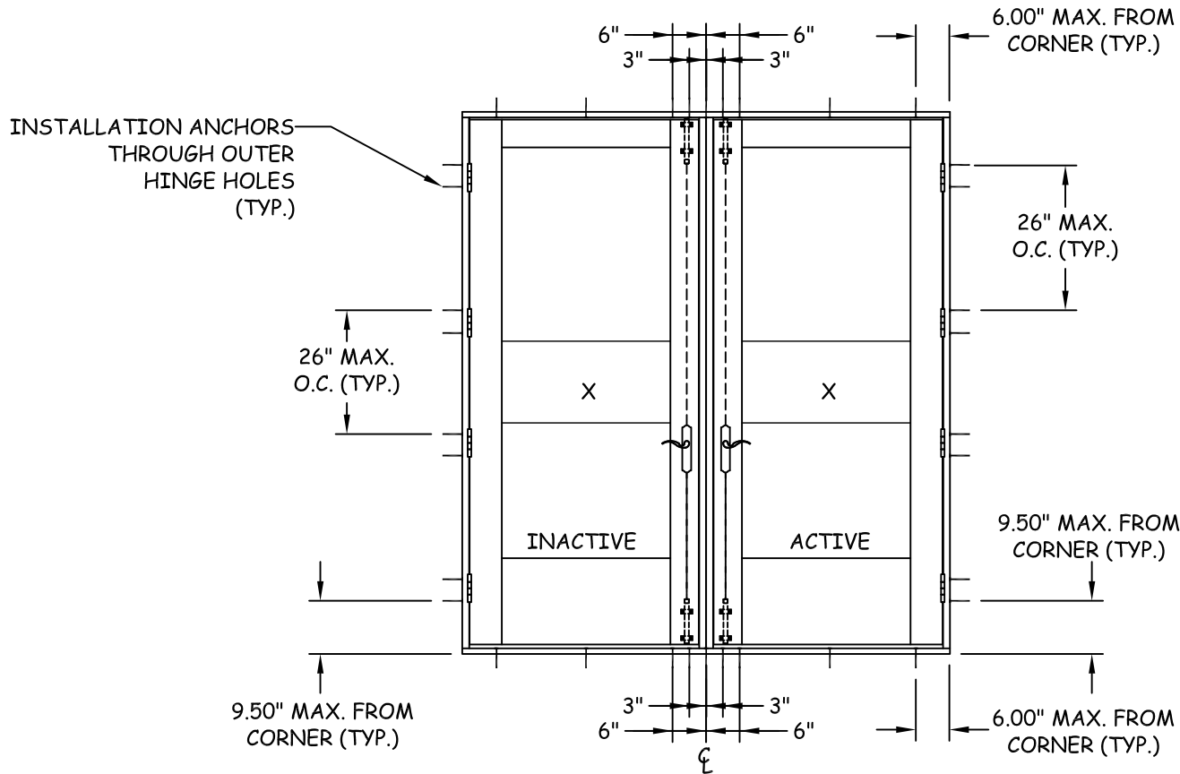
ANCHOR LAYOUT
