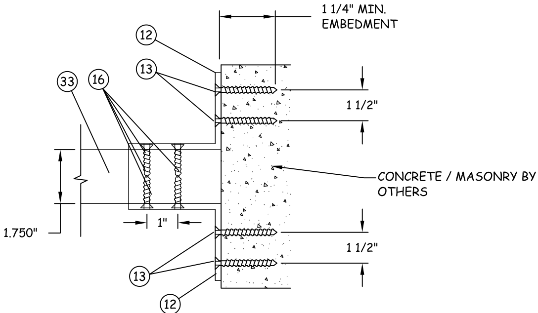
FRONT VIEW HORIZONTAL MULLION DETAIL IN CONCRETE/MASONRY
