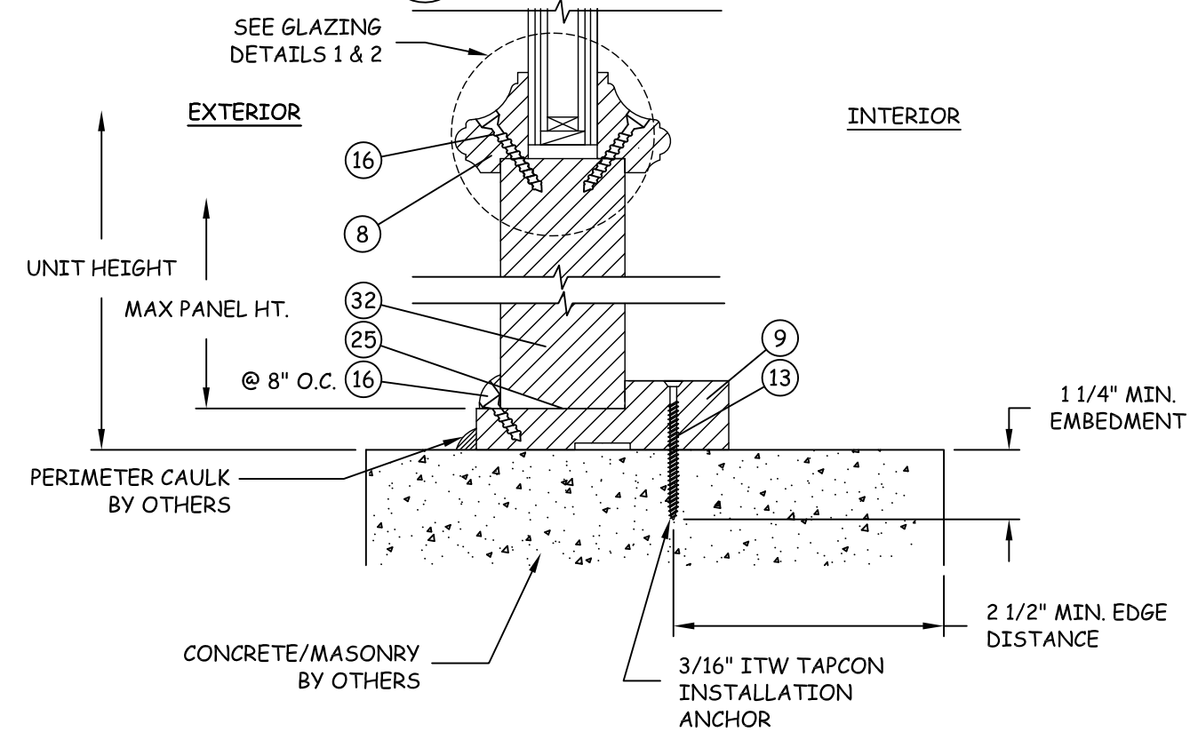
E 10 VERTICAL SECTION SIDELITE SILL - CONCRETE/MASONRY
