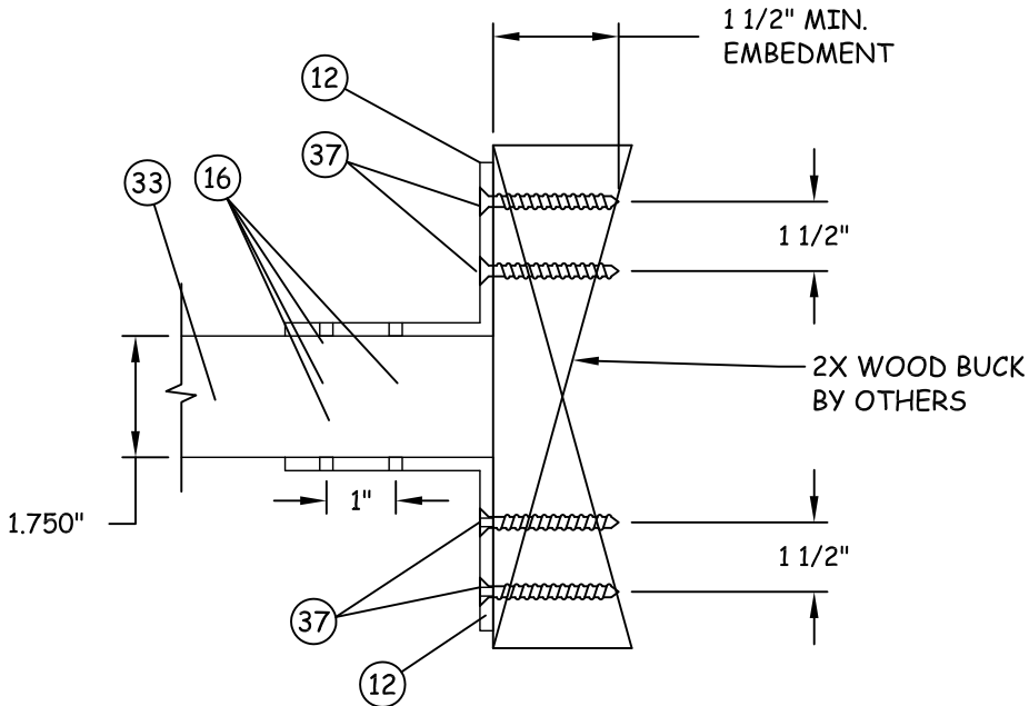
FRONT VIEW HORIZONTAL MULLION DETAIL IN 2X FRAME
