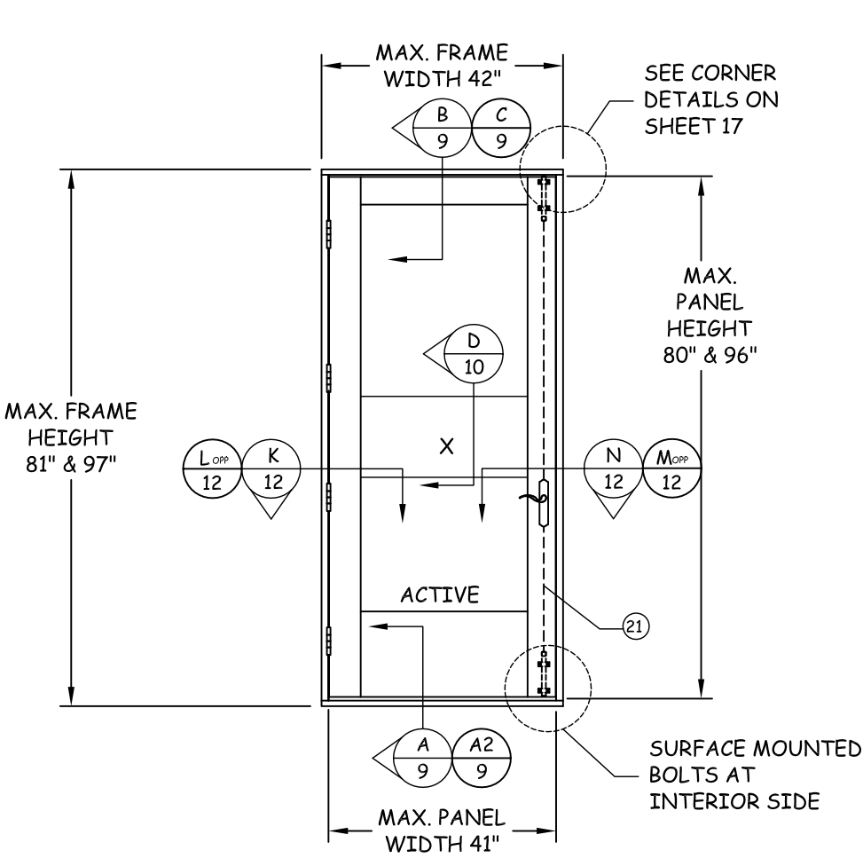
X CONFIGURATION SEE DESIGN PRESSURE TABLE EXTERIOR ELEVATION OUTSWING SINGLE OPAQUE DOOR
