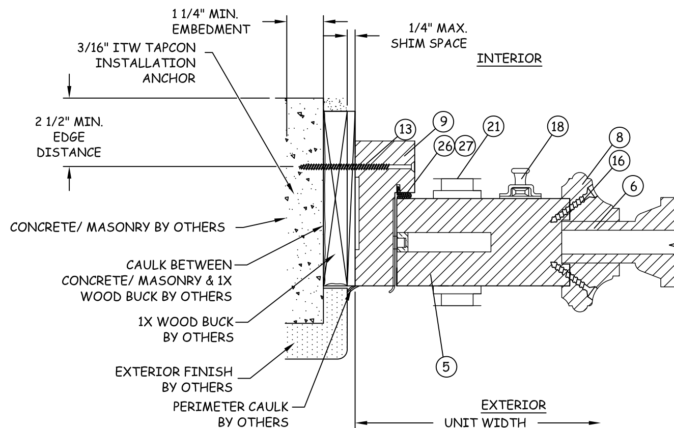
M 12 HORIZONTAL SECTION LOCK JAMB AT CONCRETE/MASONRY
